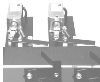
Figure 1-8: Parts manipulators (flippers)
